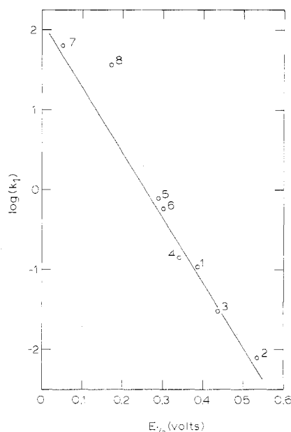
Figure 1. \log k_1 vs. E_{1/2} for various ruthenium(II) amines. Numbering corresponds to numbering in Table V. Line drawn for \log k_1 \propto 1/2 \log K_{\text{eq}} .
